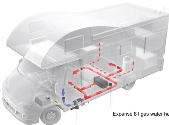
Air Top Evo 40 or Air Top Evo 55 diesel cabin air heater
